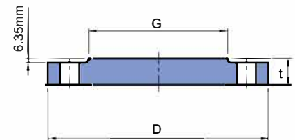
BLIND
