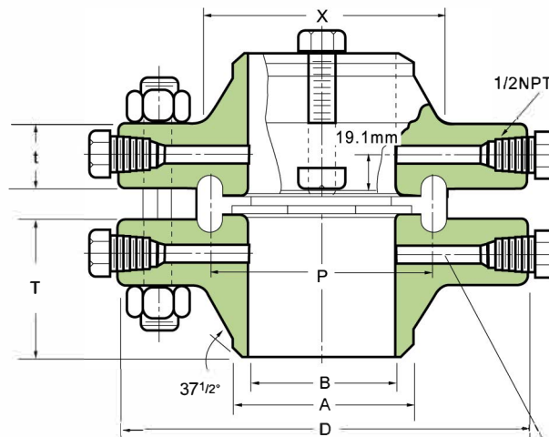
WELDING NECK (RING-TYPE JOINT)
