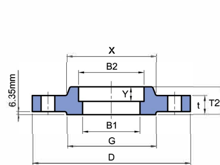
SOCKET WELDING
