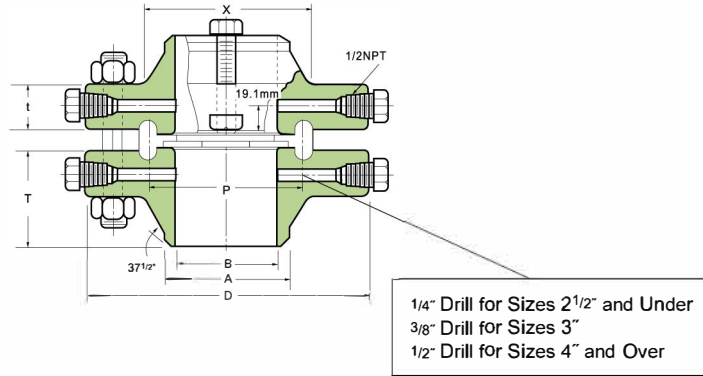
WELDING NECK (RING-TYPE JOINT)
