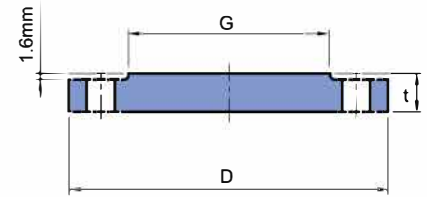
BLIND
