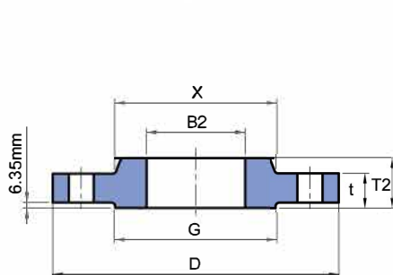
SLIP-ON
