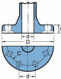
SOLID FLANGE
