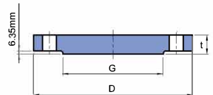
BLIND
